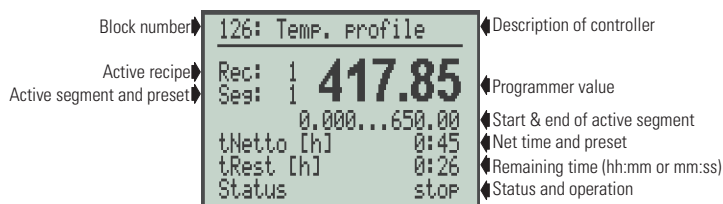
Fig. 3 Operating display for an analog programmer (APROG)
