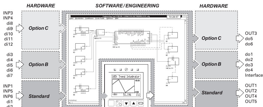
Fig. 8 Electrical connections
