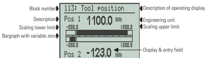
Fig. 6 Horizontal bargraph display (VBAR)
