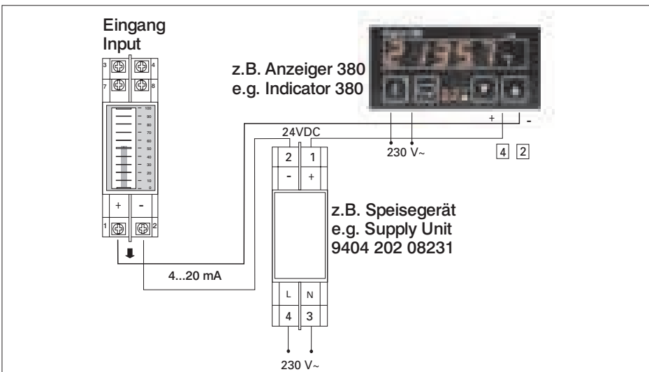
Fig. 7 Two wire connections
