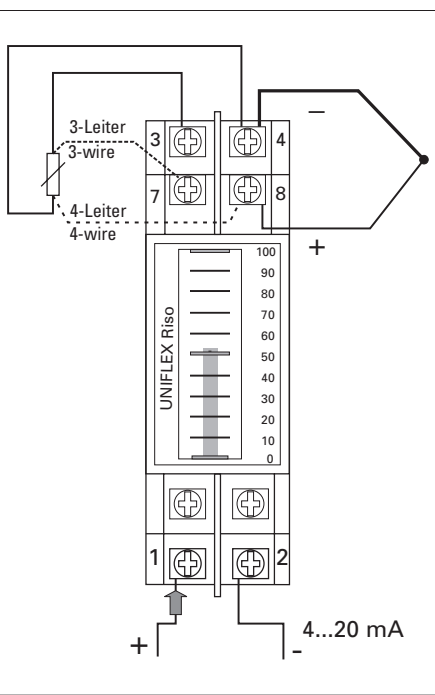
Fig. 3 Connections
