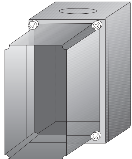
Fig. 8 Field housing IP 67
